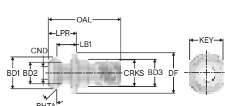
Design 2 = With through coolant
