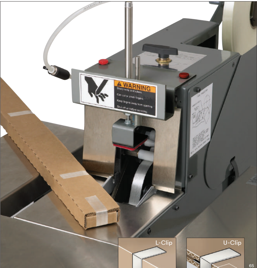
3M-Matic™ L-Clip Applicator S867 with optional U-Clip adapter.
